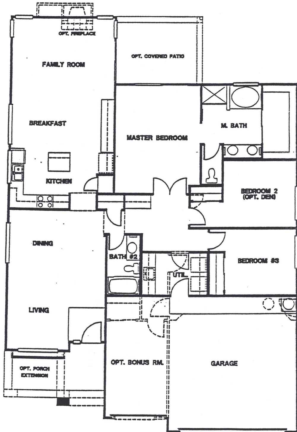
PRELIMINARY FLOOR PLAN 1744 SQ. FT. (BASIC)
