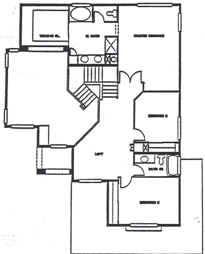
PRELIMINARY SECOND FLOOR PLAN
