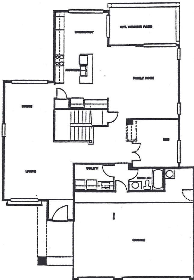
PRELIMINARY FIRST FLOOR PLAN 2681 SQ. FT.
